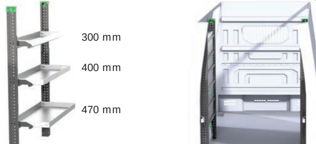
Shelf frames 0° - Shelves 0°, locking hook 90°
